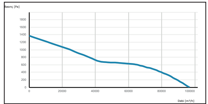
K-CAXI 1120-8-45
