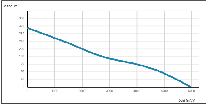
K-CAXI 500-5-25
