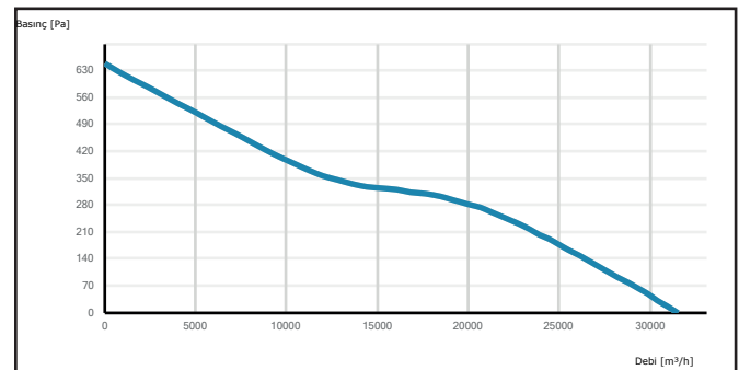
K-CAXI 800-5-35
