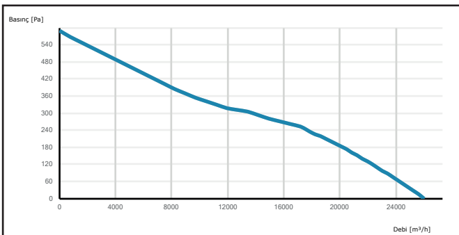
K-CAXI 800-5-30
