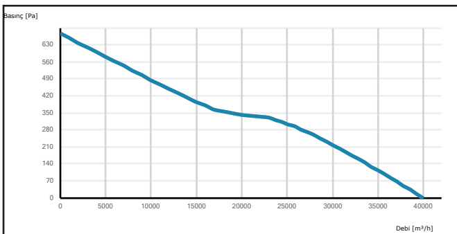
K-CAXI 900-5-35
