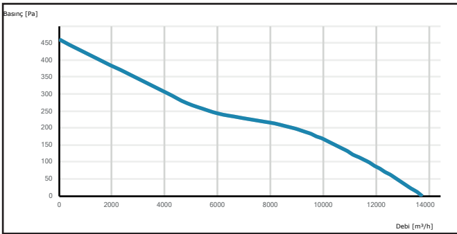
K-CAXI 630-5-30
