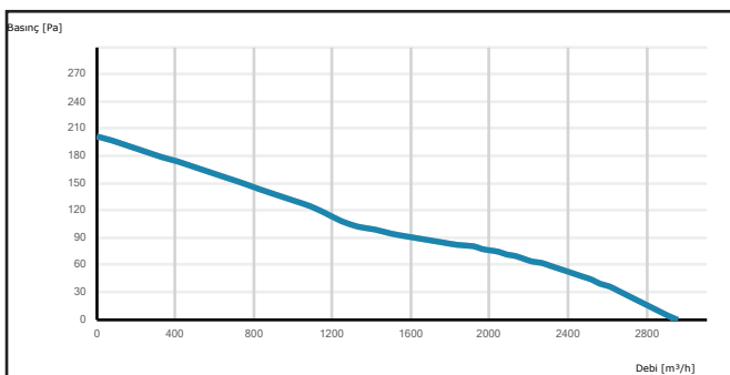
K-CAXI 400-5-25
