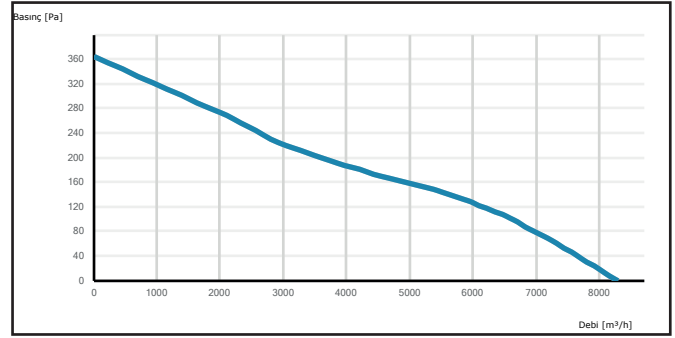
K-CAXI 560-5-25
