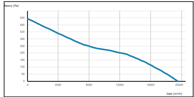
K-CAXI 710-5-30
